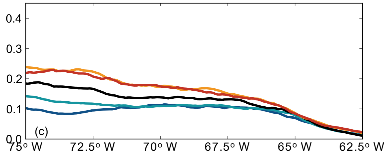
Shear from temperature gradients ( 10^{-3} \text{ s}^{-1} )
