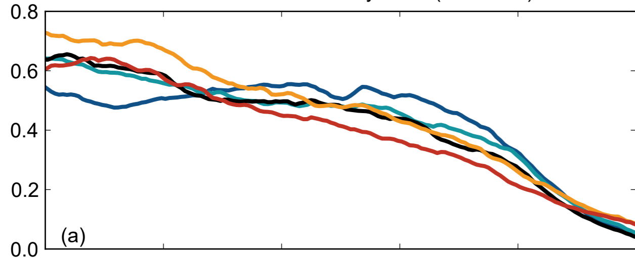
Shear from velocity field ( 10^{-3} \text{ s}^{-1} )
