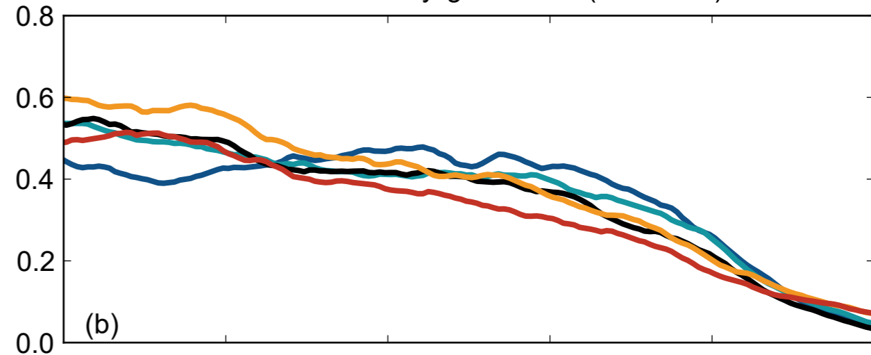
Shear from density gradients ( 10^{-3} \text{ s}^{-1} )
