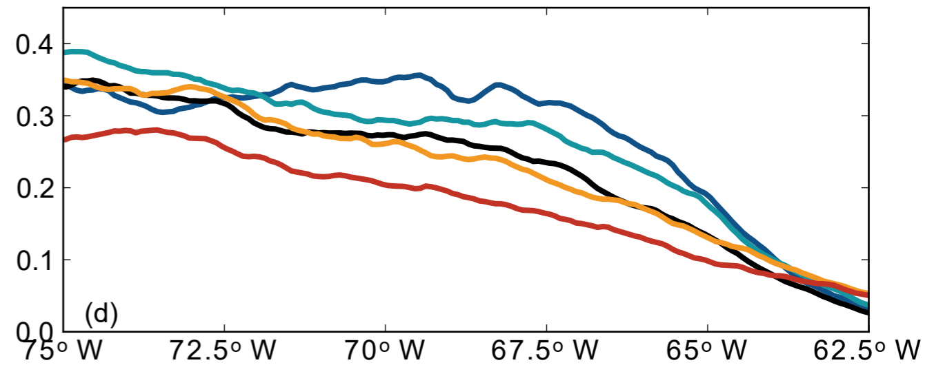
Shear from salinity gradients ( 10^{-3} \text{ s}^{-1} )
