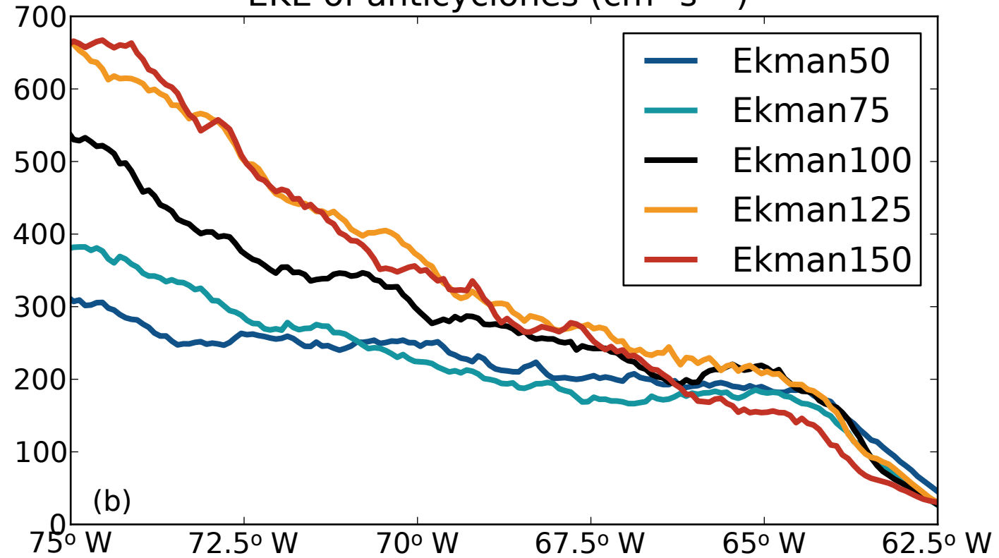
EKE of anticyclones ( \text{cm}^2 \text{s}^{-2} )
