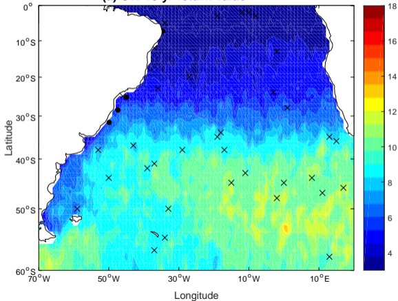
(a) GW 10-yr return value
