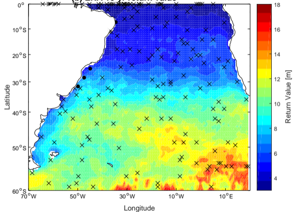
(b) ERA 10-yr return value
