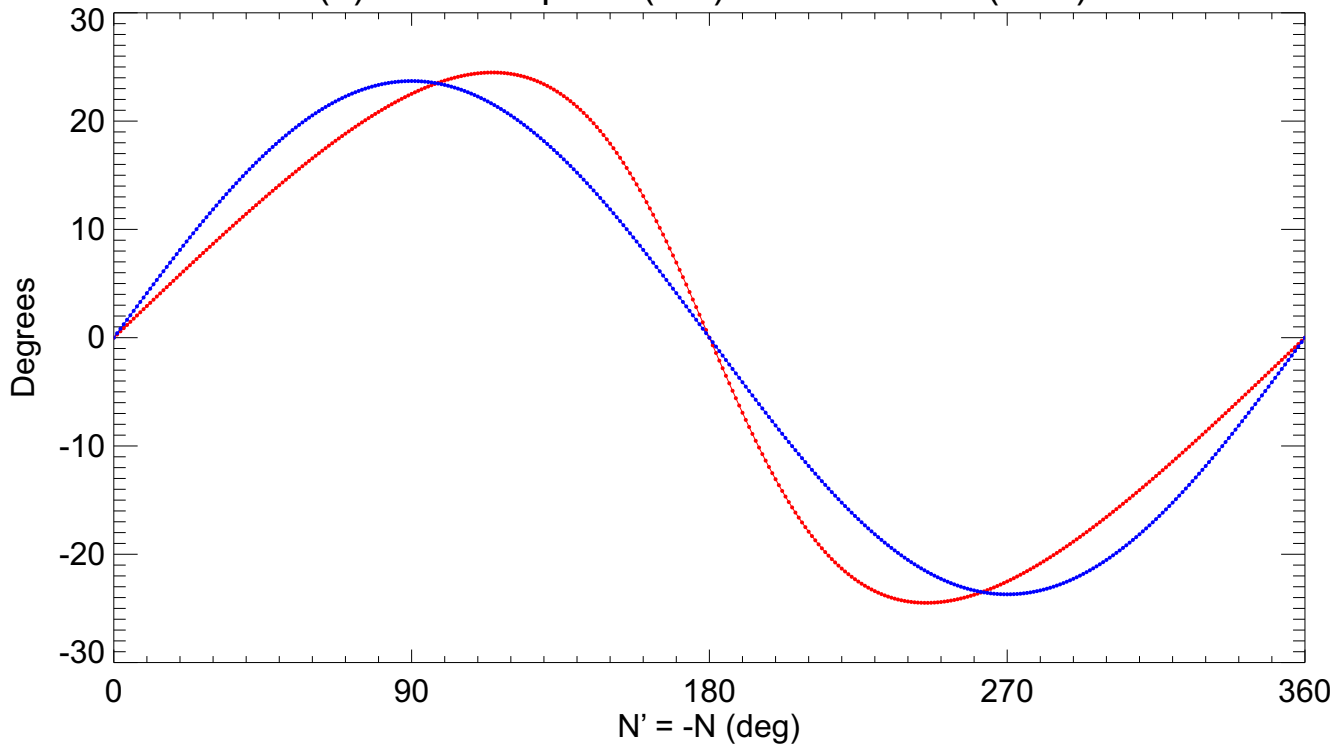
(b) u from Eq. A6. (red) and Doodson (blue)
