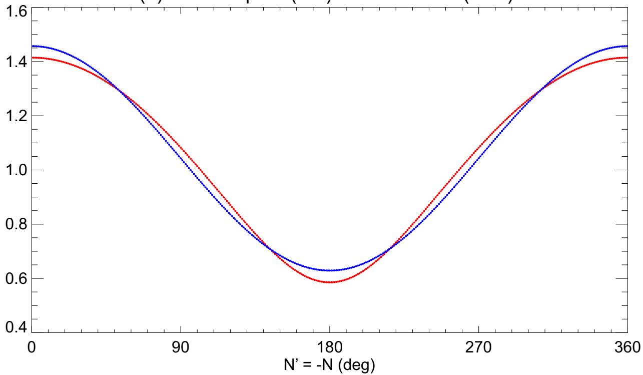
(a) f from Eq. A2 (red) and Doodson (blue)
