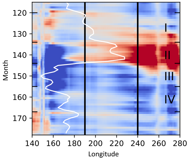
(b) B_r anomalies and MaNI
