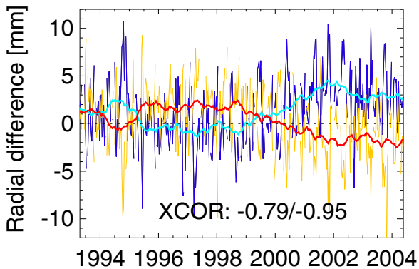
Geoid-GRGS
