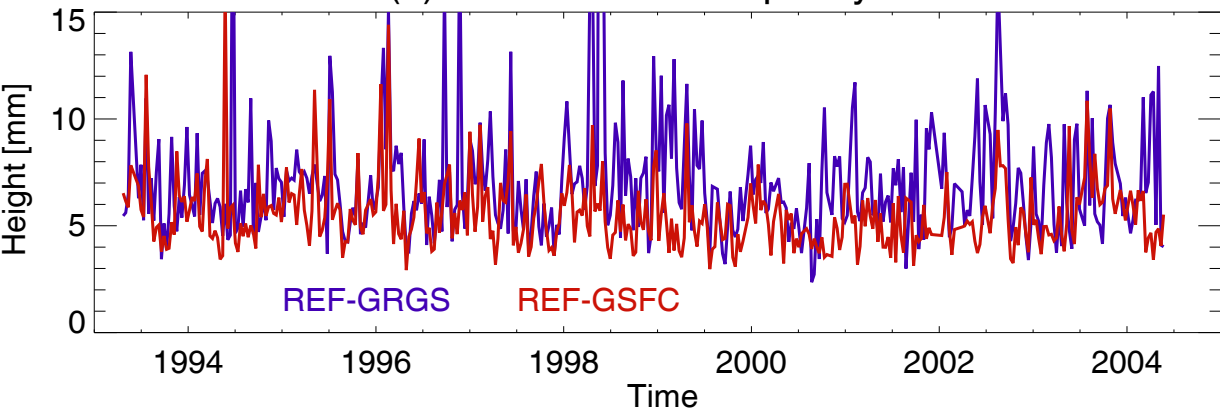
(a) Global mean rms per cycle
