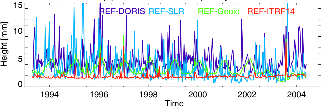
(b) Global mean rms per cycle
