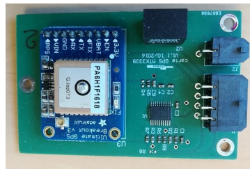
GPS board
