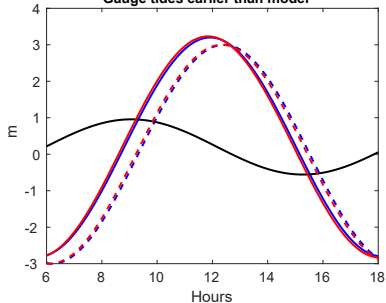
Gauge tides earlier than model
