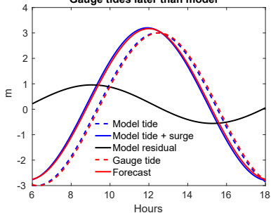
Gauge tides later than model
