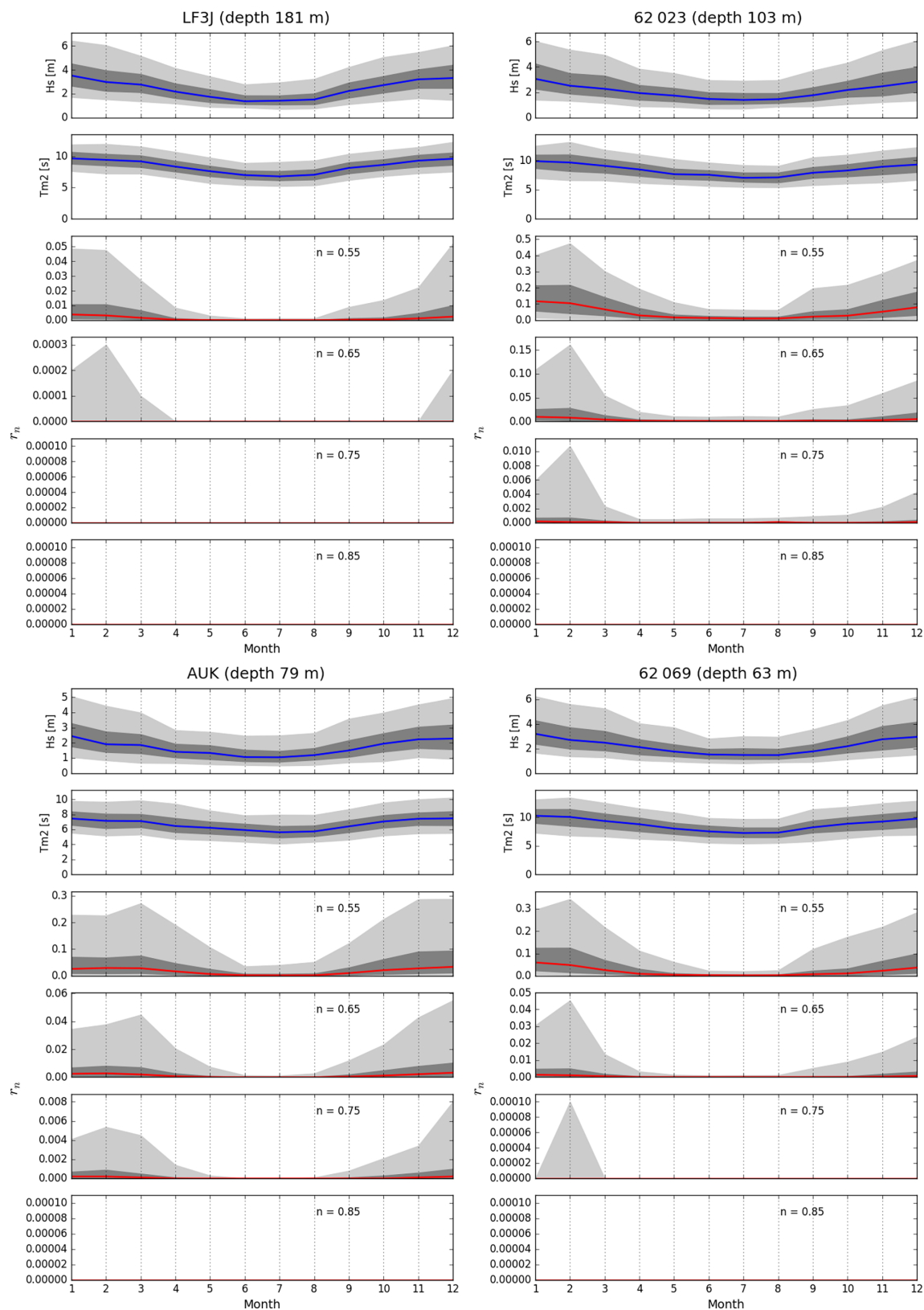
Figure 3. Monthly values of significant wave height, mean period, and r_n values for n = 0.55, 0.65, 0.75 , and 0.85 at stations LF3J, 62023, AUK, and 62069. Median values are given by red and blue lines; 25th to 75th percentiles are shown as dark gray; 5th to 95th percentiles are shown as light gray.
