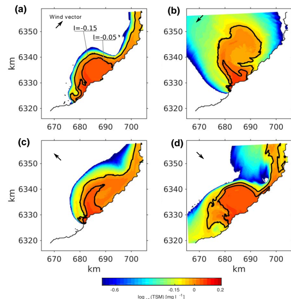
Figure 6. Instantaneous surface TSM concentration maps for simulation with uniform ambient density and a constant wind speed of 4 \text{ m s}^{-1} blowing in a downstream (a), upstream (b), offshore (c) and onshore (d) direction at 6T from the start of the simulation. Solid lines represent TSM concentrations of \log_{10}(\text{TSM}) = -0.15 and -0.05 . The coordinate system is on the UTM-34v projection.
