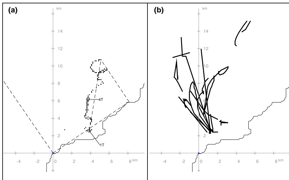
Figure 10. The trajectories of the bulge centre for the idealized simulation (a) and the realistic simulation (b) from 24 March 2007 05:00 to 5 April 2007 00:00. Each dot shows the location of the bulge centre at hourly intervals. Dashed lines show the normal and tangent to the coastline, the distance of the bulge centre from the location at 1T up to the end of the simulation, and the distance of the bulge centre at the end of the simulation to the coast in the direction of the normal to the coast. 1T and 4T show the location of the bulge centre after one and four rotation periods of the earth starting from 24 March 2007 05:00 (a). Discontinuities in the bulge trajectories for the realistic model simulation exist because the bulge centre was defined only if anti-cyclonic circulation with closed streamlines was present (b).
