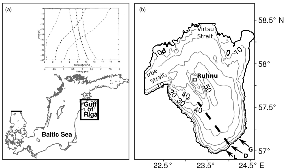
Figure 1. Map showing the location of the Gulf of Riga in the Baltic Sea (a). Embedded are mean (bold) temperature (dashed) and salinity (dash dotted) profiles with standard deviations (thin) from the central Gulf of Riga (adopted from Raudsepp, 2001). Topography of the Gulf of Riga (b). Arrows mark river mouth locations for the Daugava (D), Lielupe (L) and Gauja (G) rivers. The square shows the location of the weather station. The bold dashed line shows the transect of ferry-box measurements used for the model validation.
