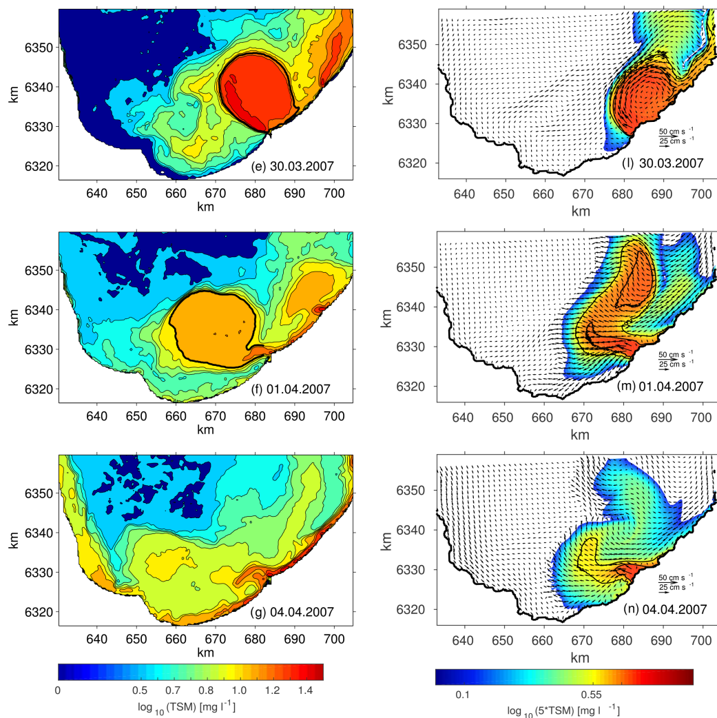
Figure 4. TSM concentration maps for the southern part of the Gulf of Riga from satellite images (left column) and TSM concentration and surface velocity maps from the numerical simulation (right column). The bold contours on the satellite images show the indicative edge of the Daugava River bulge. Black contours on the numerical model simulation maps represent TSM concentrations of \log_{10}(\text{TSM}) = -0.15 and -0.05 . The former is used for the determination of the Daugava River bulge. The coordinate system is on the UTM-34v projection (Cont.).
