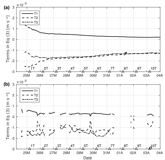
Figure 9. Time series of spatially averaged momentum balance terms (see Eq. 3): centrifugal term ( T1 ) (solid), Coriolis term ( T2 ) (dashed), and pressure gradient term ( T3 ) (dash dotted) for ideal (a) and real (b) bulges. Triangles represent the rotation period of the earth starting from 24 March 2007, 05:00.
