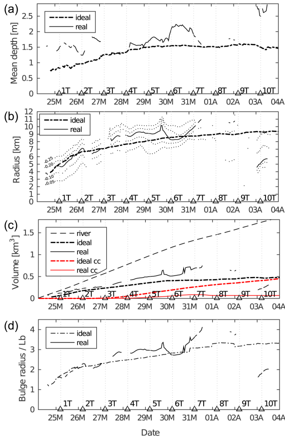
Figure 7. Time series of the Daugava River bulge mean depth (a), bulge radius (b), bulge volume (c) and the bulge effective radius scaled with the bulge Rossby radius (d). The solid line represents the real model simulation and the dash-dotted line the idealized model simulation. Time series of the bulge radius where the bulge is defined: I = \log_{10}(\text{TSM}) > -0.05 ; -0.10 ; -0.20 ; -0.25 (dotted) (b). Time series of cumulative river water (dashed), bulge volume (black) and volume of the coastal current (red) in the real model simulation (solid) and ideal model simulation (dash-dotted) (c). Triangles represent the rotation period of the earth starting from 24 March 2007 05:00 GTM.
