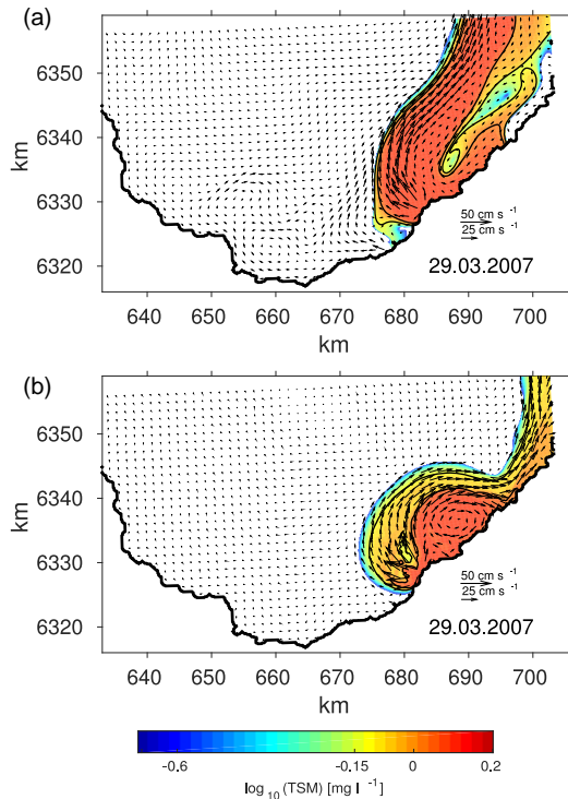
Figure 5. Instantaneous surface velocity and TSM concentration maps for simulation with realistic ambient density and no wind forcing (a) and idealized model simulation with uniform ambient density and no wind forcing (b) at noon on 29 March 2007. Solid lines represent TSM concentrations of \log_{10}(\text{TSM}) = -0.15 and -0.05 . The coordinate system is on the UTM-34v projection.
