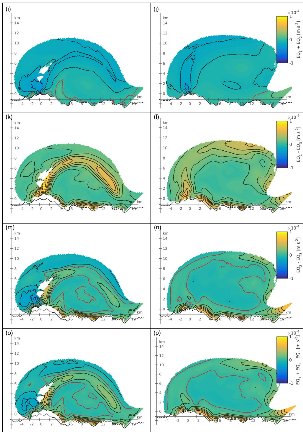
Figure 8. Bulge depth and depth averaged velocities, the terms ( T_1 , T_2 , T_3 ) of the balance (see Eq. 3) and the combinations of the terms for idealized (left column) and realistic (right column) model simulations on 29 March 2007 at 20:00. Bulge depth and depth averaged velocities (a–b), centrifugal term ( T_1 ) (c–d), Coriolis term ( T_2 ) (e–f), pressure gradient term ( T_3 ) (g–h), T_1 + T_2 (i–j), T_1 - T_2 (k–l), T_2 - T_3 (m–n) and T_1 + T_2 - T_3 (o–p). The contour interval is 1 \text{ m s}^{-2} . The red isoline represents zero. The blank area within the bulge is where the tracer concentrations were below the threshold values of the bulge definition (see text for bulge definition). The origin of the coordinate system is at the mouth of the Daugava River. True north is shown with the arrow (Cont.).
