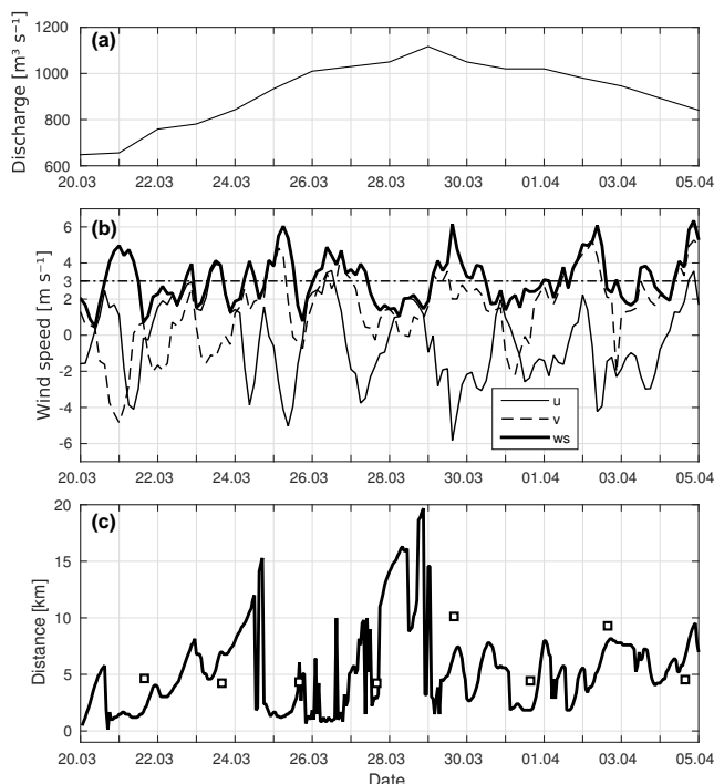
Figure 3. Time series of (a) daily mean Daugava River discharge; (b) 3 h wind speed (bold), eastern (solid) and northern (dashed) wind components from the HIRLAM-ETA data set at Ruhnu, and 3 \text{ m s}^{-1} wind speed (dash dotted); (c) offshore location of the maximum salinity gradient from model (solid) and ship measurements (open square) for the period from 20 March to 5 April 2014. Distance is measured along the ship track from the mouth of the Daugava River.
